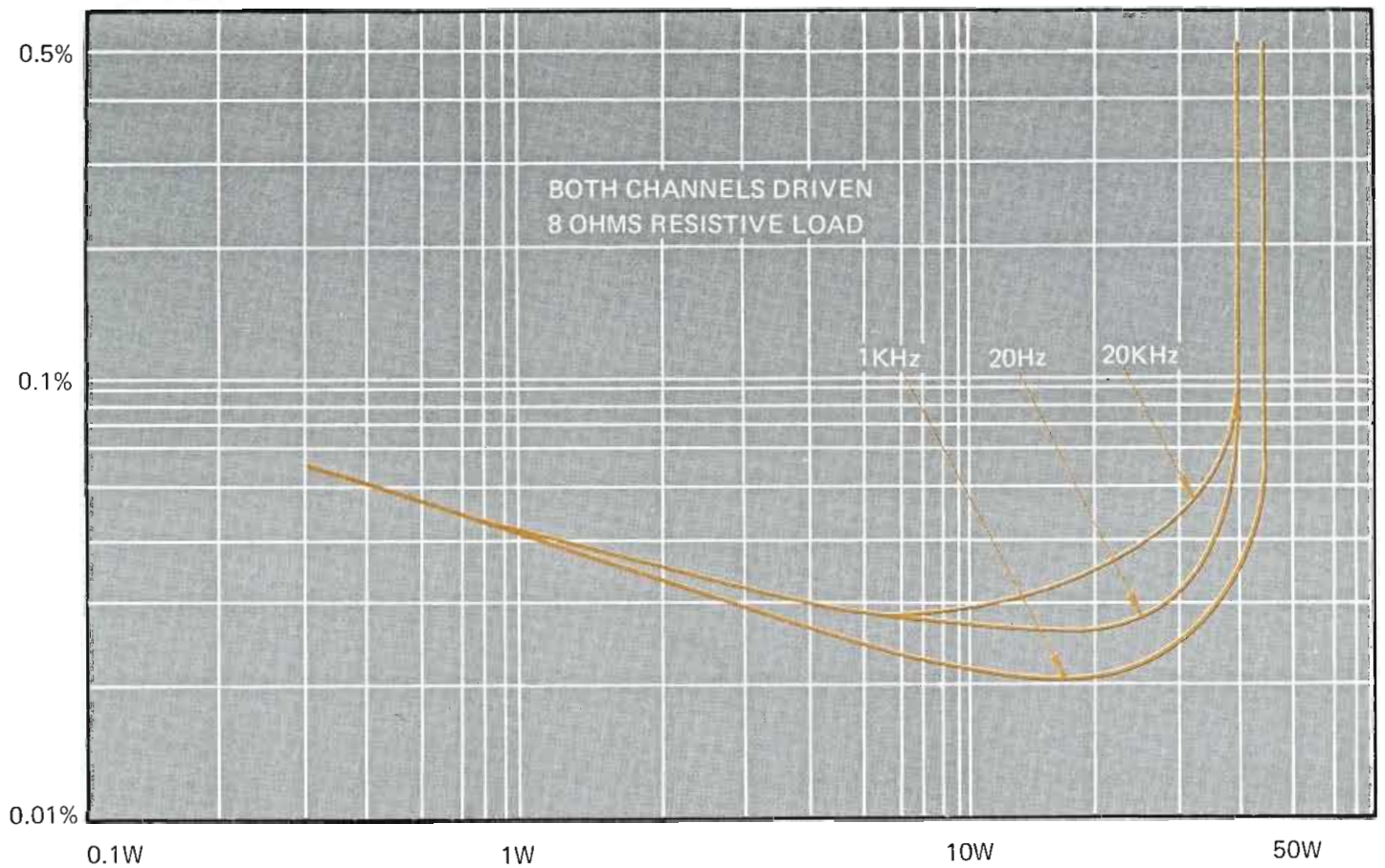
Figure 10. Distorsion harmonique
